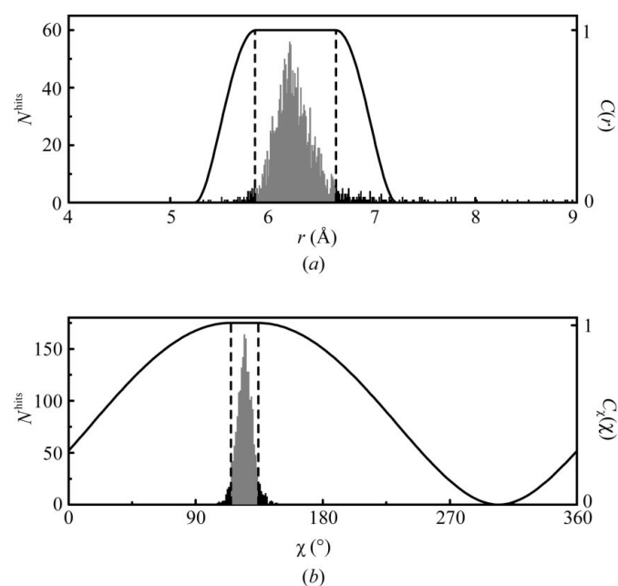
Figure 2 Observed distributions N_{\text{hits}} and defined conditions C for interatomic distance r and (b) N_{\text{hits}} and C_\chi for torsion angle \chi between the outermost atoms of a linear element comprising atoms C^\alpha(i) to C^\alpha(i + 4) in an \alpha -helical conformation. The minimum and maximum values for which C = 1 are set to comprise 90% of the observed conformations (shown in grey).
