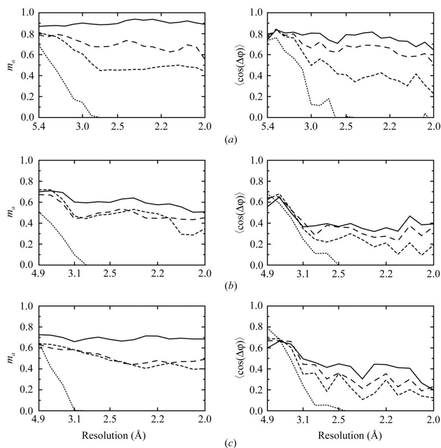
Figure 8 Estimated figures of merit m_a and average cosine of the phase error, \langle \cos(\Delta\phi) \rangle , for the (a) all- \alpha helical (1i2t), (b) all- \beta sheet (3ebx) and (c) mixed \alpha/\beta (1ds3) test cases. Values are shown as calculated for the initial scrambled structures (dotted lines), structures after optimization cycle 1 (dashed lines) and cycle 2 (long-dashed lines) and for the final optimized structures (solid lines).
