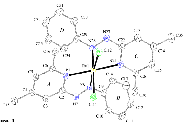
Figure 1 View of the Ru(dazpy) 2 Cl 2 complex located on a general position, with the atom and ring numbering schemes. Displacement ellipsoids for non-H atoms are drawn at the 50% probability level. H atoms have been omitted for clarity.
