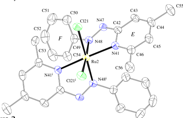
Figure 2 View of the Ru(dazpy) 2 Cl 2 complex located on a crystallographic twofold rotation axis, with the atom and ring numbering schemes. Displacement ellipsoids for non-H atoms are drawn at the 50% probability level. H atoms have been omitted for clarity. [Symmetry code: (i) -x, y, \frac{1}{2} - z .]
